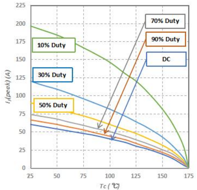
Fig.8-Current Derating
