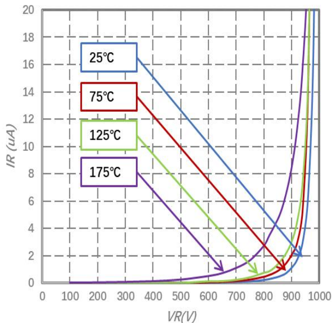
Fig.2-Typical Reverse Characteristics
